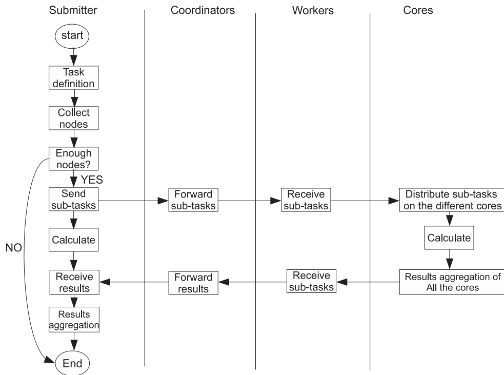
FIGURE 4 Activity diagram of a parallel application with GRIDHPC
