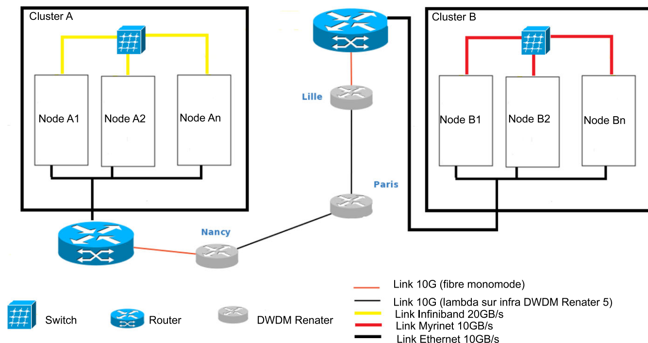
FIGURE 1 Example of multi-network distributed platform
