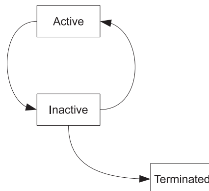
FIGURE 7 States of computing nodes in the termination detection procedure of asynchronous iterations
