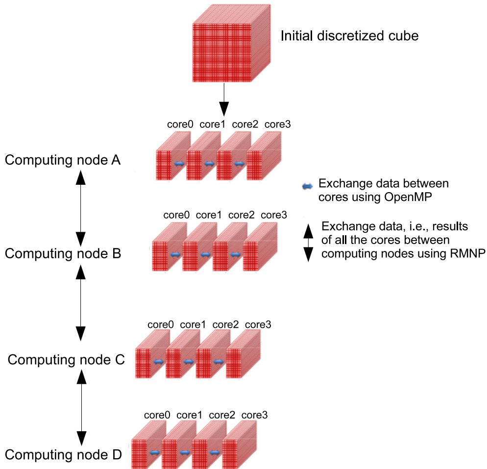
FIGURE 5 Example of decomposition of the discretized obstacle problem
