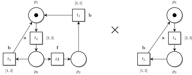
Fig. 4: Product of a TPN N_f (left) and its “twin” N_o (right) for the fault f .
