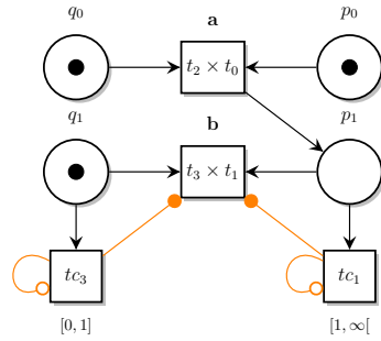
Fig. 2: Example of IPTPN
