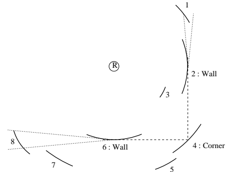
Figure 11: A set of RCDs in which a corner has been completely detected
