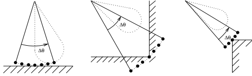
Figure 3: RCDs generated by a wall, a corner and an edge. The leftmost sonar lobe of each RCD is shown.
