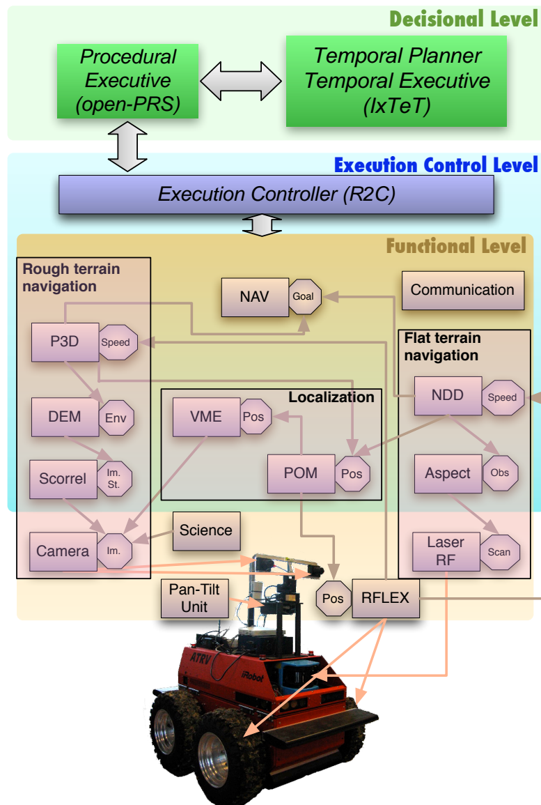
Fig. 8. An instance of the architecture with the functional level that embeds the functionalities mentioned in this section. Modules involved in the flat terrain navigation mode are on the right (mainly module Laser RF, ASPECT and NDD), and the modules involved in the 3D navigation mode are on the left (loop SCORREL, DEM, P3D). RFLEX just uses either one or the other speed reference produced. Arrows between modules indicate data flow – for readability purpose, only the main ones are shown.
