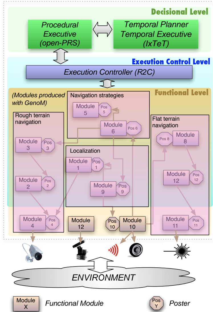
Fig. 1. The LAAS architecture. The functional level is here populated with dummy modules, to illustrate that sets of modules can be composed to provide higher modalities.
