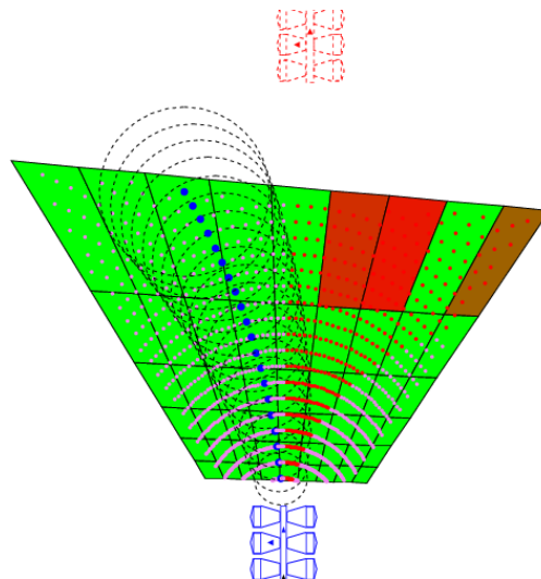
Fig. 5. Evaluation of elementary trajectories. Positions are evaluated along trajectories corresponding to various steering angles. To consider safe paths in case of trajectory deviations, the robot width is enlarged as it proceeds along the trajectory.
