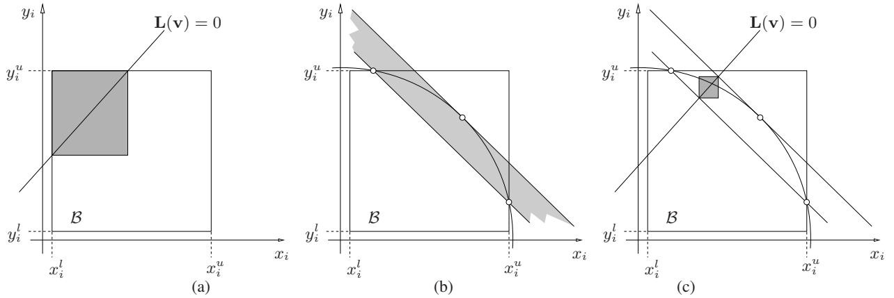
Fig. 3. (a) Shrinking \mathcal{B} to fit the linear variety \mathbf{L}(\mathbf{v}) = 0 . (b) Half-planes approximating the circular arc inside \mathcal{B} . (c) Smallest box enclosing the intersection of \mathbf{L}(\mathbf{v}) = 0 with the half-planes in (b).
