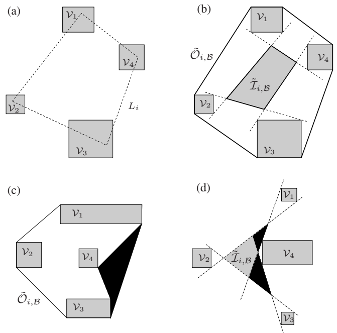
Fig. 4. (a) Bounding rectangles for the vertices of a link L_i , for a box of ambient space. (b) Inner and outer polygons of L_i for such box. (c) An outer polygon overestimating \mathcal{O}_{i,\mathcal{B}} . (d) An inner polygon underestimating \mathcal{I}_{i,\mathcal{B}} . Black regions indicate the over- and under-estimation, respectively.
