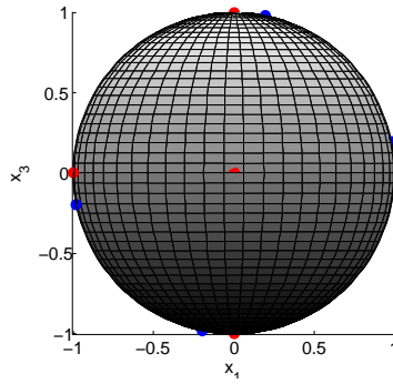
FIGURE 8. Support points recovered in Example 6.6 for the D -optimal design and d = 1 (red) and the points which are recovered when additionally fixing some moments as described in Subsection 6.7 (blue).
