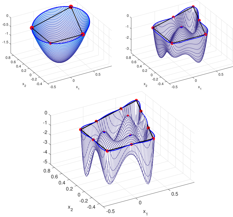
FIGURE 3. The polynomial p_d^* - \binom{2+d}{2} where p_d^* denotes the Christoffel polynomial of Example 6.2 for d = 1 (top left), d = 2 (top right), d = 3 (bottom middle). The red points correspond to the \binom{2+d}{2} -level set of the Christoffel polynomial.
