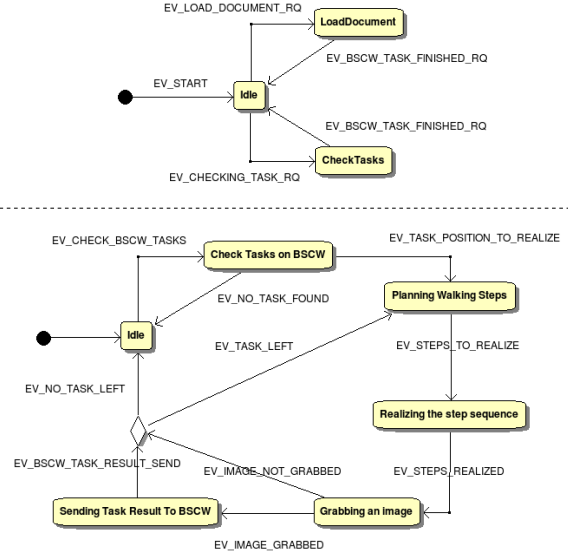
Fig. 4 Statechart model of the case study
