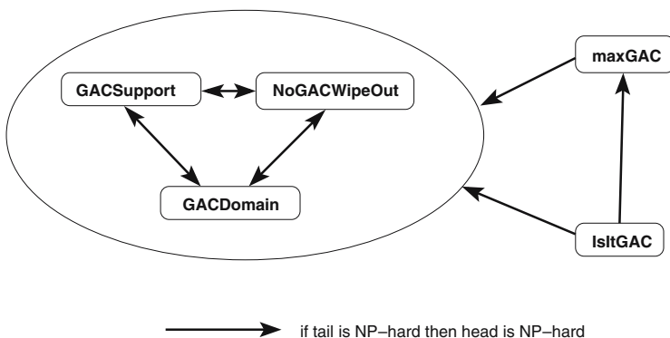
Fig. 1 Summary of dependencies between intractable problems
