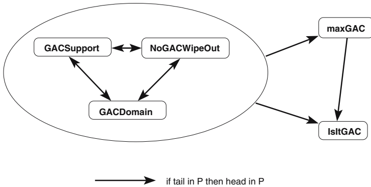
Fig. 2 Summary of the dependencies between tractable problems
